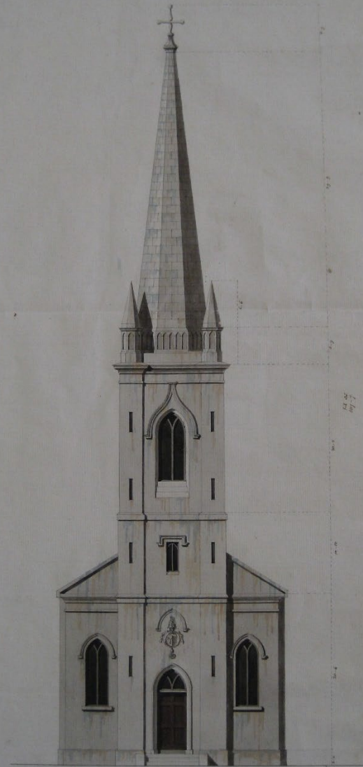
Elevation of West front
